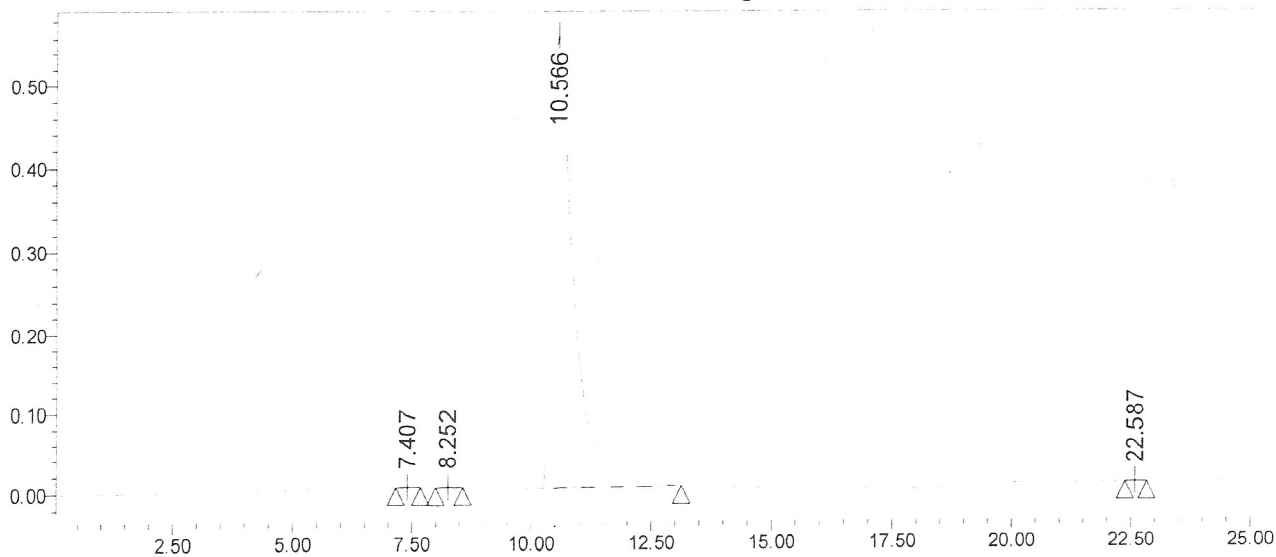
Auto-Scaled Chromatogram
